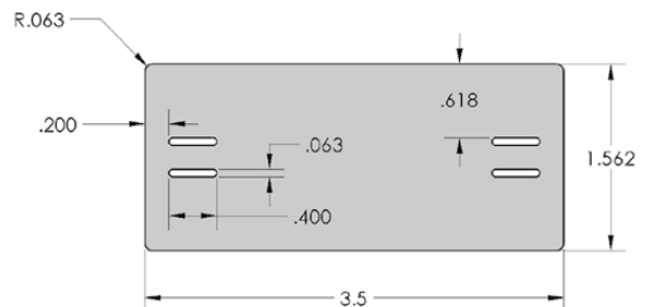
Hole Code 4RL : (4) .062" x .400" Slots
