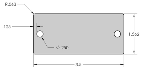
Hole Code 225 : (2) .250"Ø Holes
