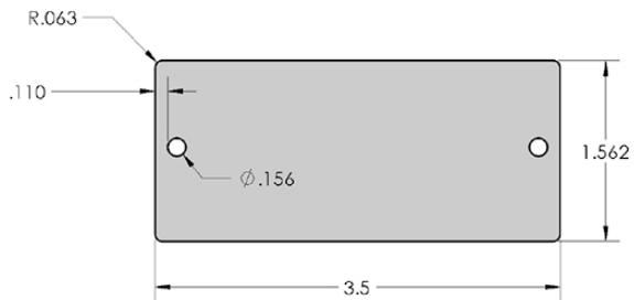
Hole Code 215 : (2) .156"Ø Holes
